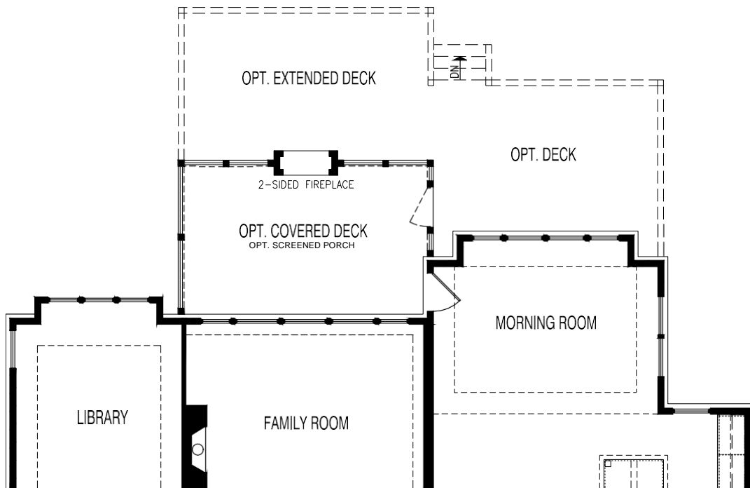
First Floor Plan w/ Optional Covered Deck & Optional Deck Conditions
