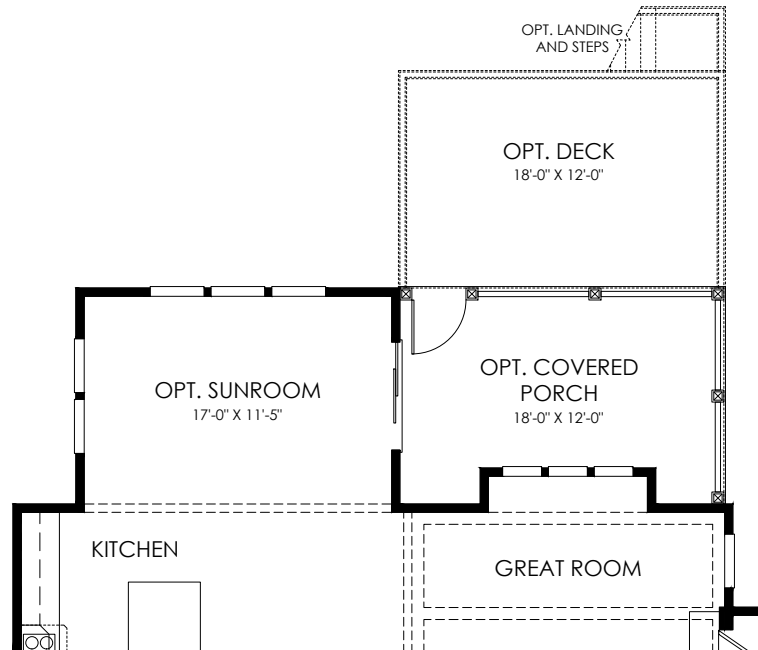
PART. FIRST FLOOR W/ OPTIONAL SUNROOM W/ COVERED PORCH
