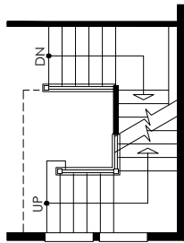
OPTIONAL OPEN RAILING TO BASEMENT STAIRS
