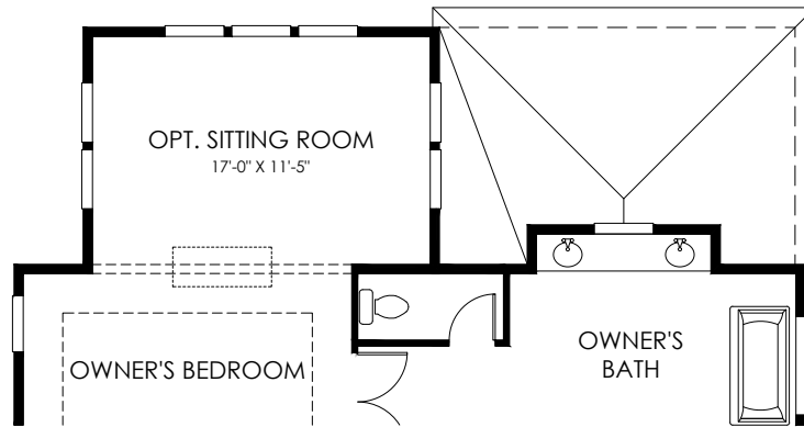
PART. SECOND FLOOR W/ OPTIONAL SUNROOM W/ COVERED PORCH
